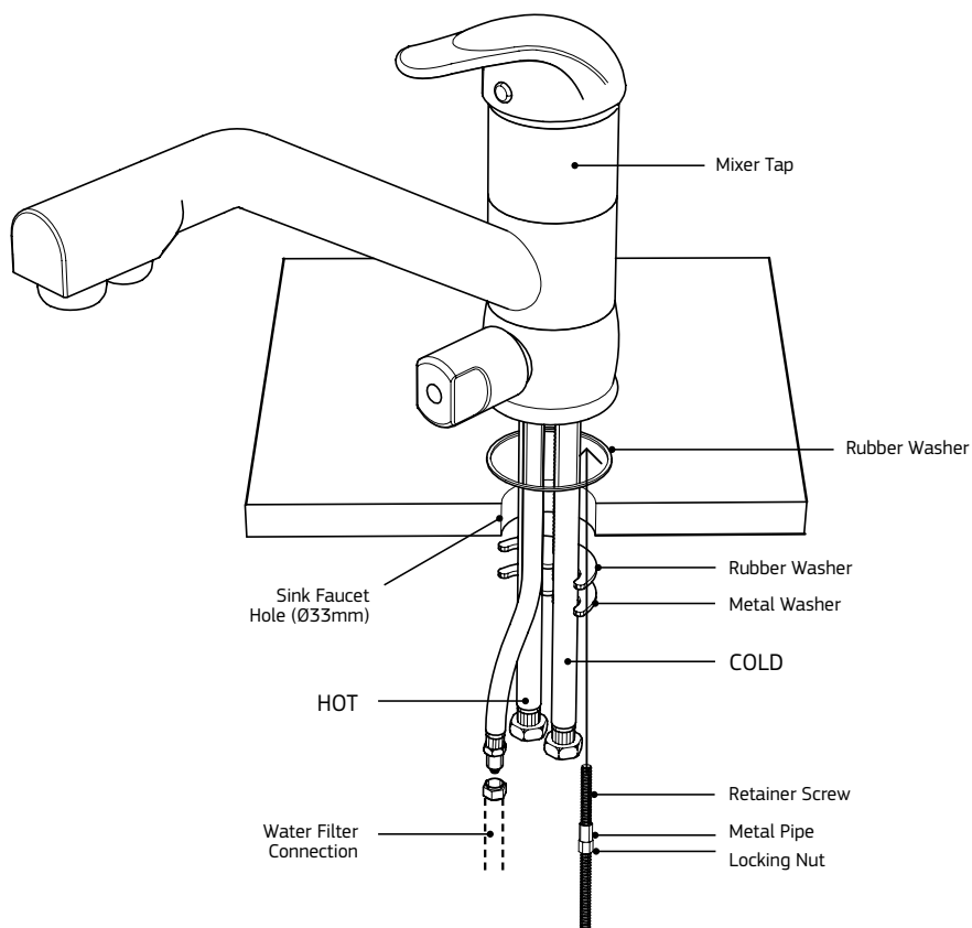
Fig. 1 - Mixer Tap Installation Guide
