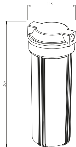
FP 10" HOUSINGS
