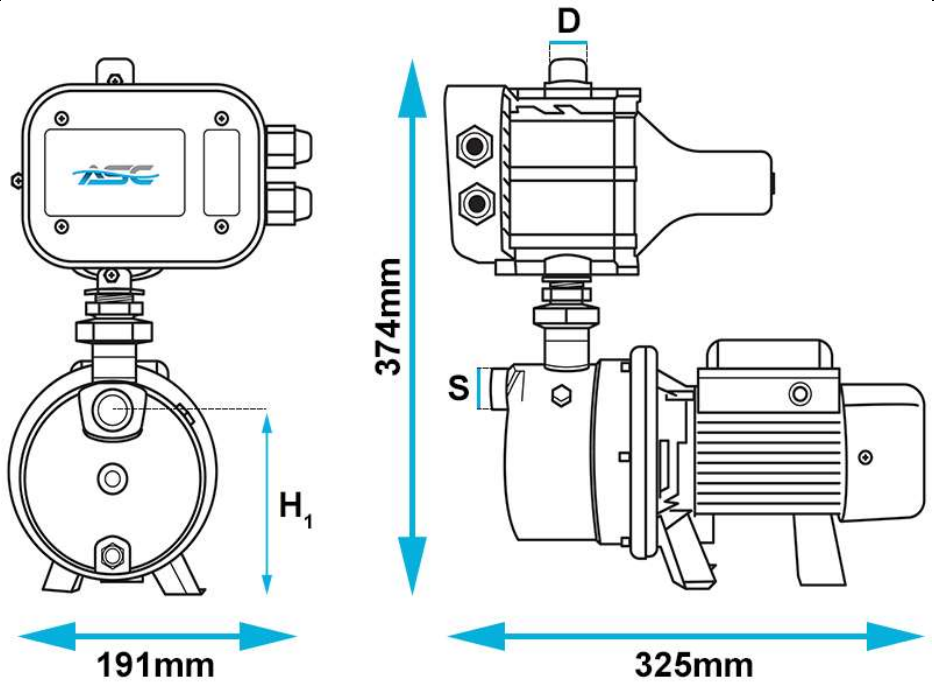
1 ASC-J35/50 2 ASC-J40/60 3 ASC-J48/65 4 ASC-J50/100
