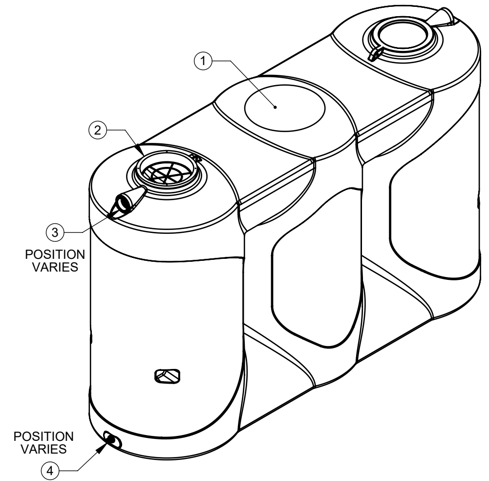
ISOMETRIC VIEW
