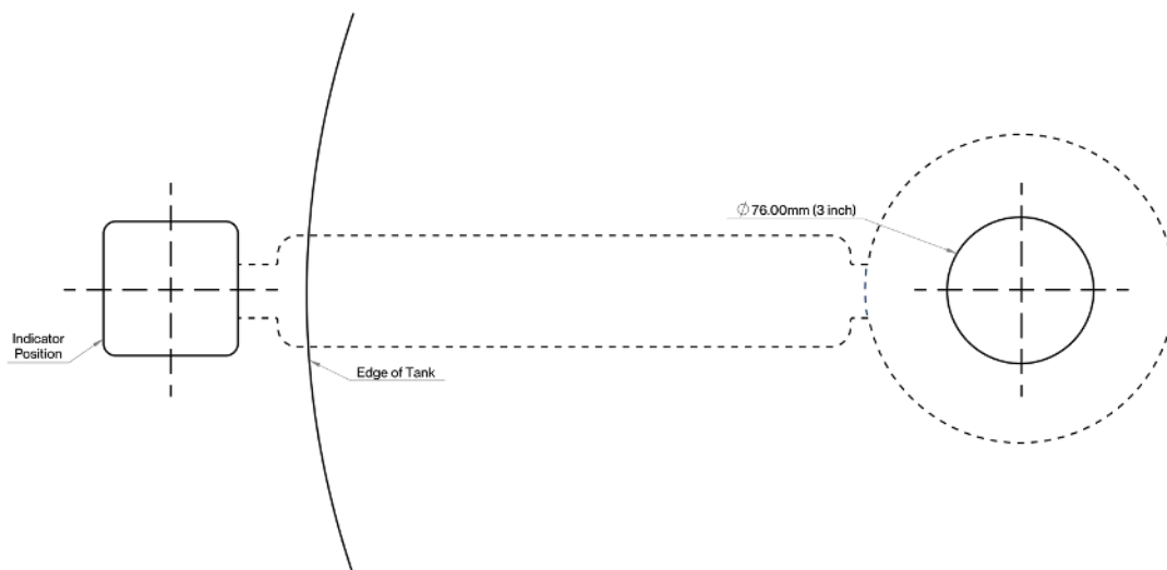
Side Wall Guided Tank Gauge Box
